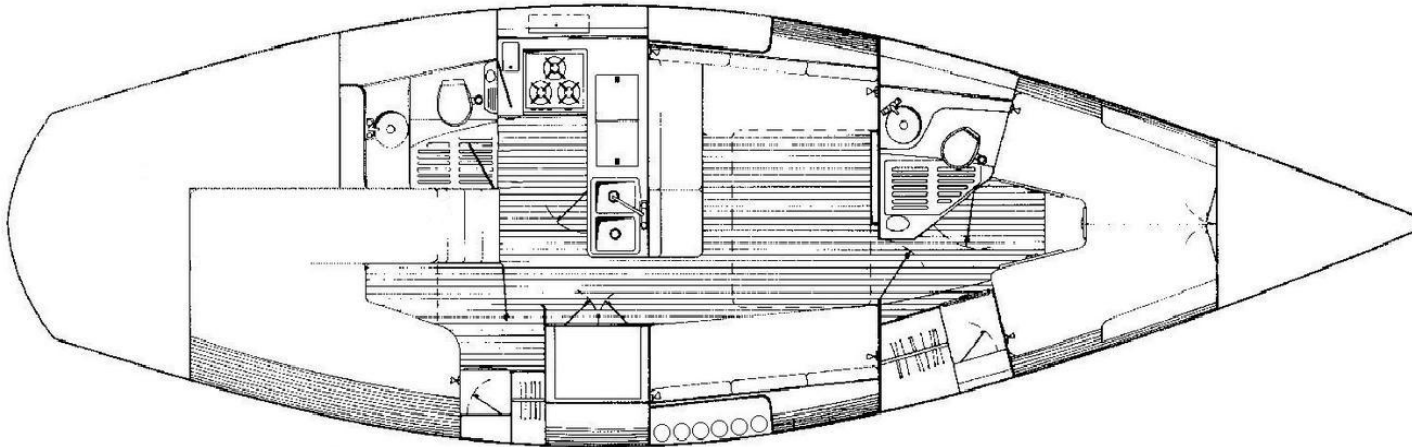
J/40 Interior Layout
